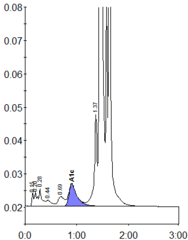
Peak table - ID: 10445783
